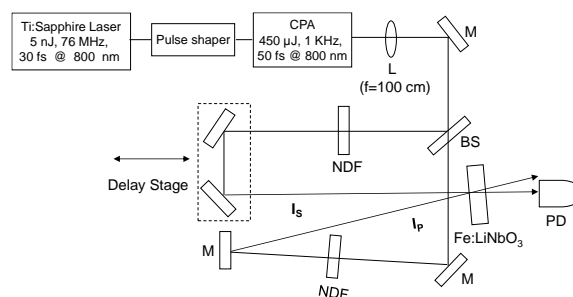
Fig. 1. Experimental setup.
